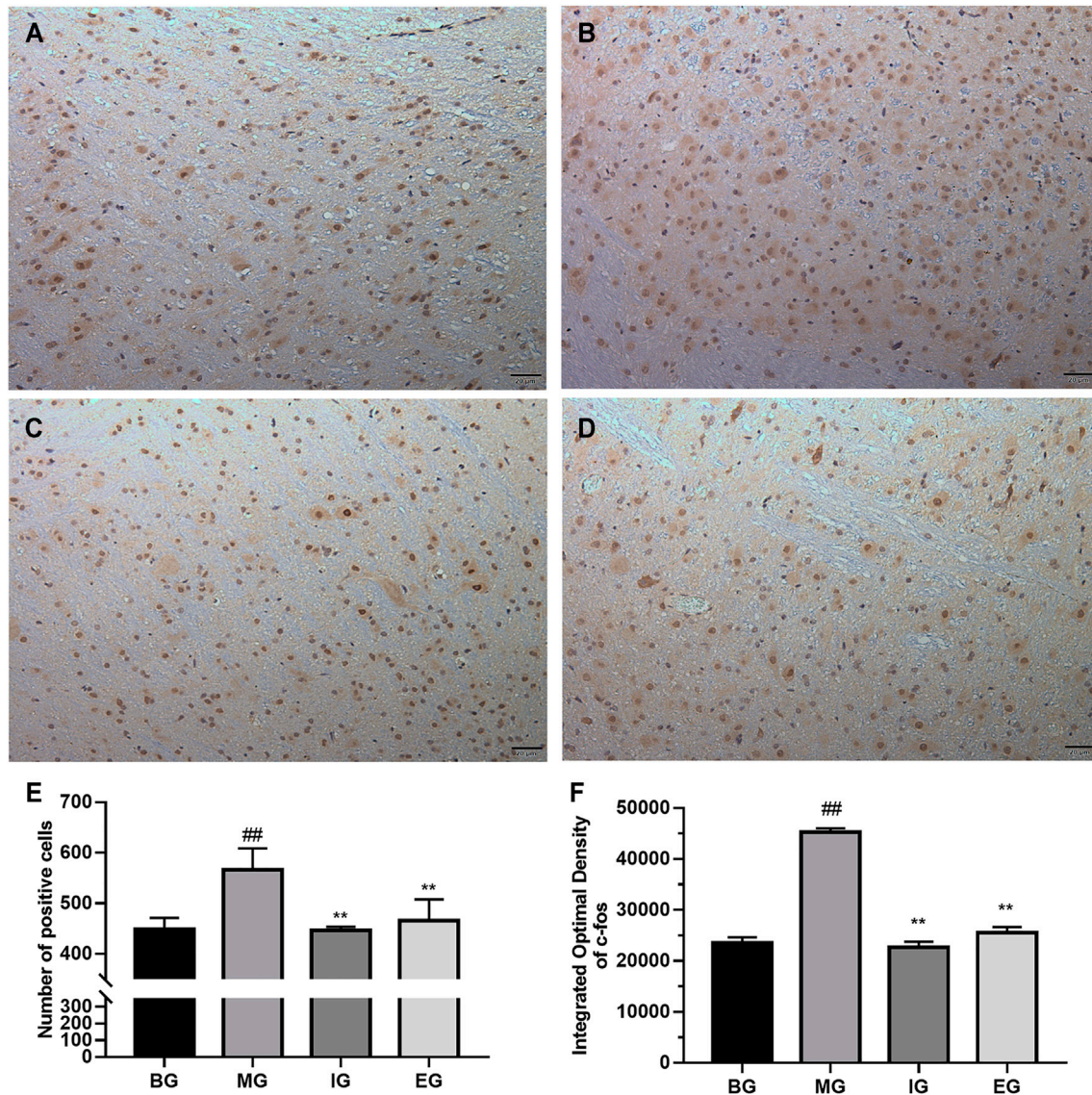
FIGURE 5 | The response of emodin on c-Fos neurons in the brainstem after NTG stimulation (sagittal cut). Immunohistochemistry photos: (A) BG, (B) MG, (C) IG, (D) EG; bar graph: (E) the number of c-Fos positive cells; (F) Integral Optical Density (IOD); taken photos under microscope at 200× magnification: Scale bar = 20 μm; values were represented as the mean ± SD ( n = 5 ). ## p < 0.01 vs. the blank, ** p < 0.01 vs. the model.
